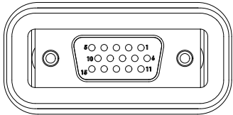
DB15 FEMALE SCALE 1.000
